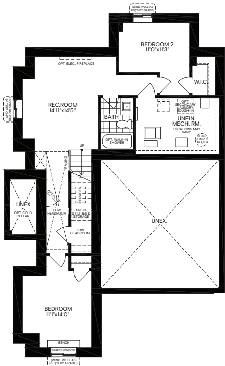
5 Basement Package 2 Bedroom Plan
