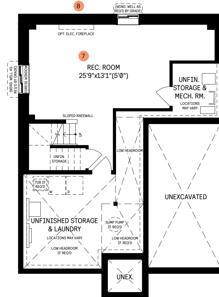
BASEMENT
