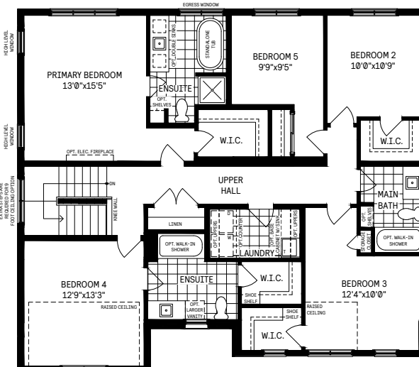
3 5 Bedroom Plan*
