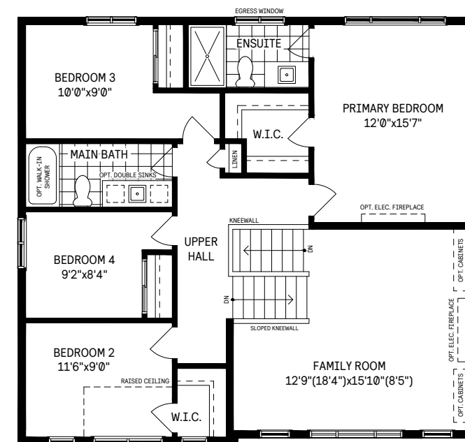
2 4 Bedroom Plan*
