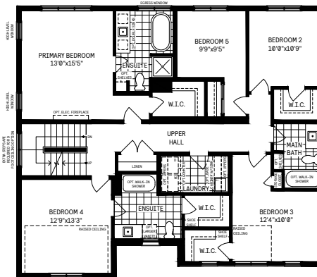
3 5 Bedroom Plan*
