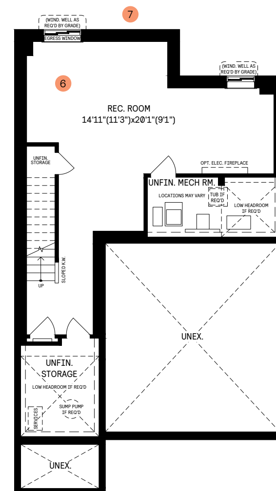
BASEMENT
