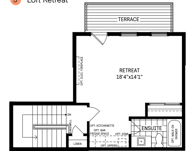
5 Loft Retreat
