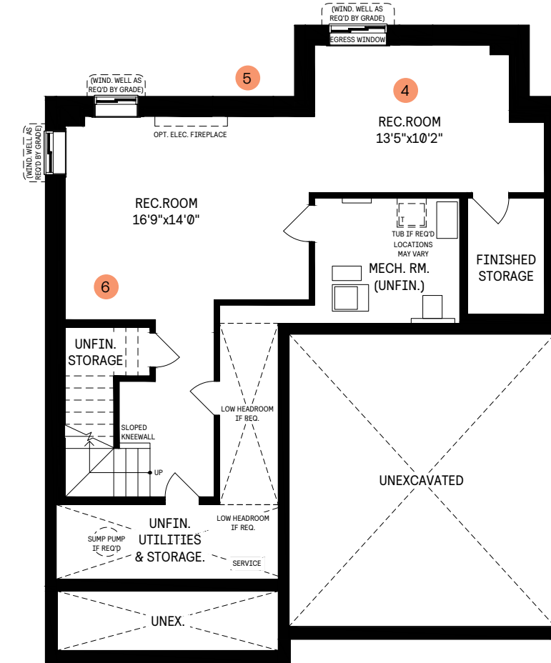
BASEMENT
