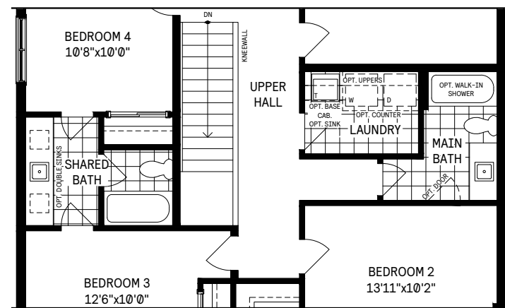
2 Shared Bath
