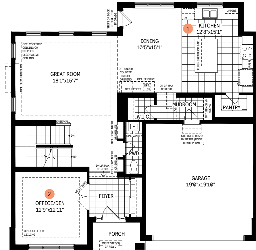
MAIN FLOOR
