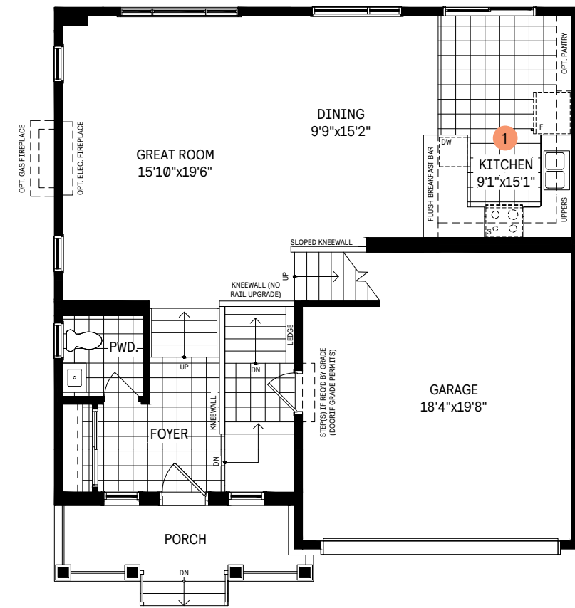
MAIN FLOOR
