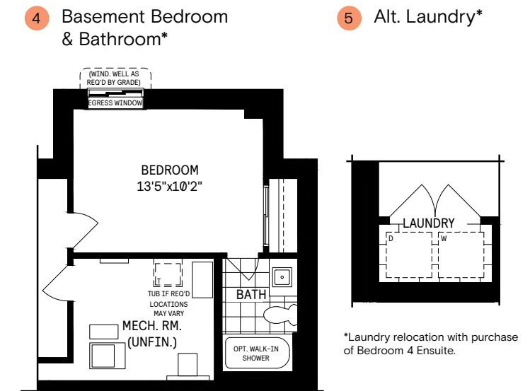
BASEMENT – DESIGNER CHOICE OPTIONS
