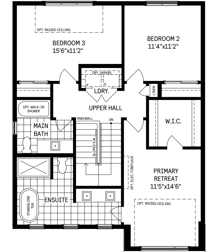
4 Primary Retreat*
