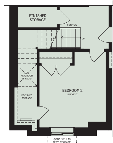
10 Finished Basement Secondary Suite 2 Bedrooms
