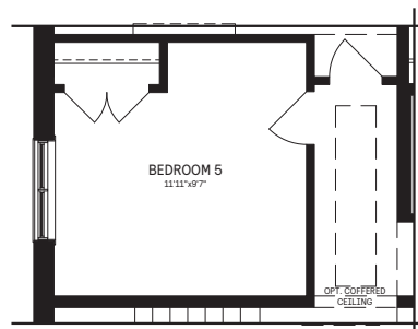
6 5 Bedroom Plan
