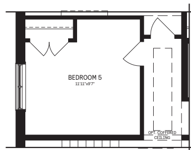
9 5 Bedroom Plan
