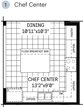
MAIN FLOOR - DESIGNER CHOICE OPTIONS
