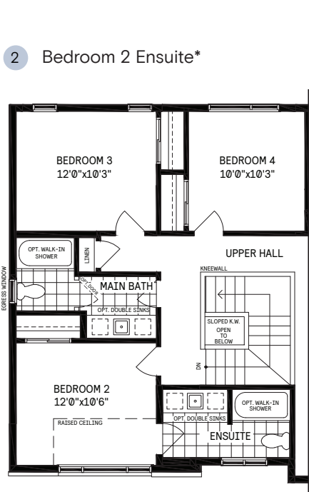
SECOND FLOOR – DESIGNER CHOICE OPTIONS
