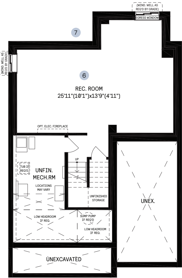
BASEMENT
