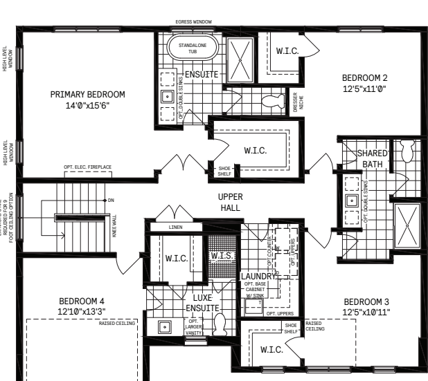
4 Alt. Second Floor*
