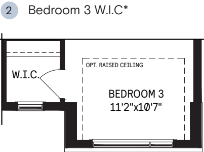
SECOND FLOOR - DESIGNER CHOICE OPTIONS
