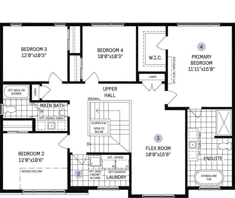
SECOND FLOOR
