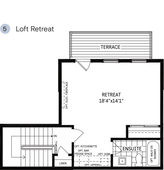
LOFT – DESIGNER CHOICE OPTIONS
