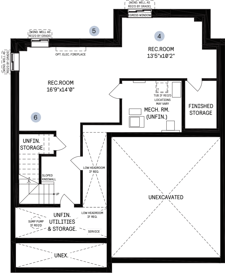
BASEMENT
