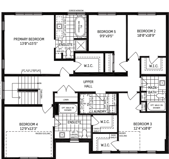
3 5 Bedroom Plan*
