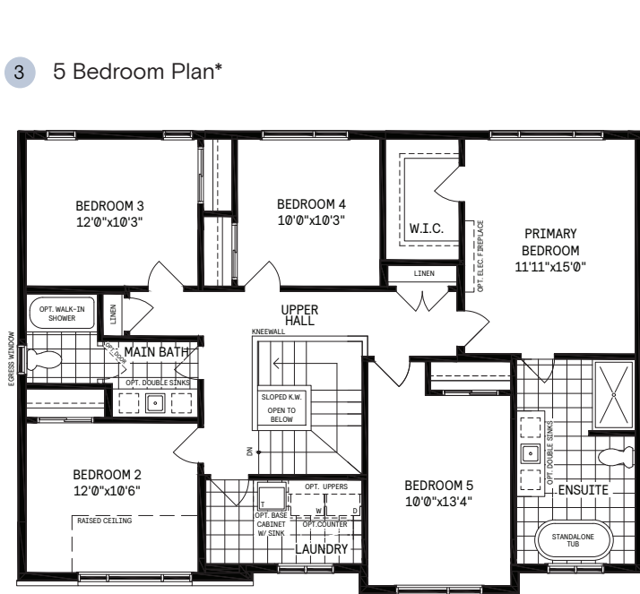
5 Bedroom Plan*
