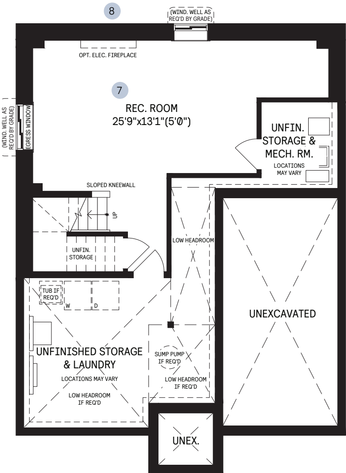
BASEMENT
