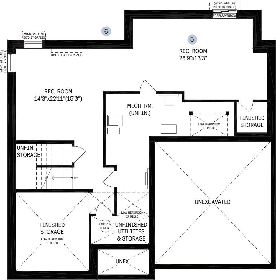
BASEMENT
