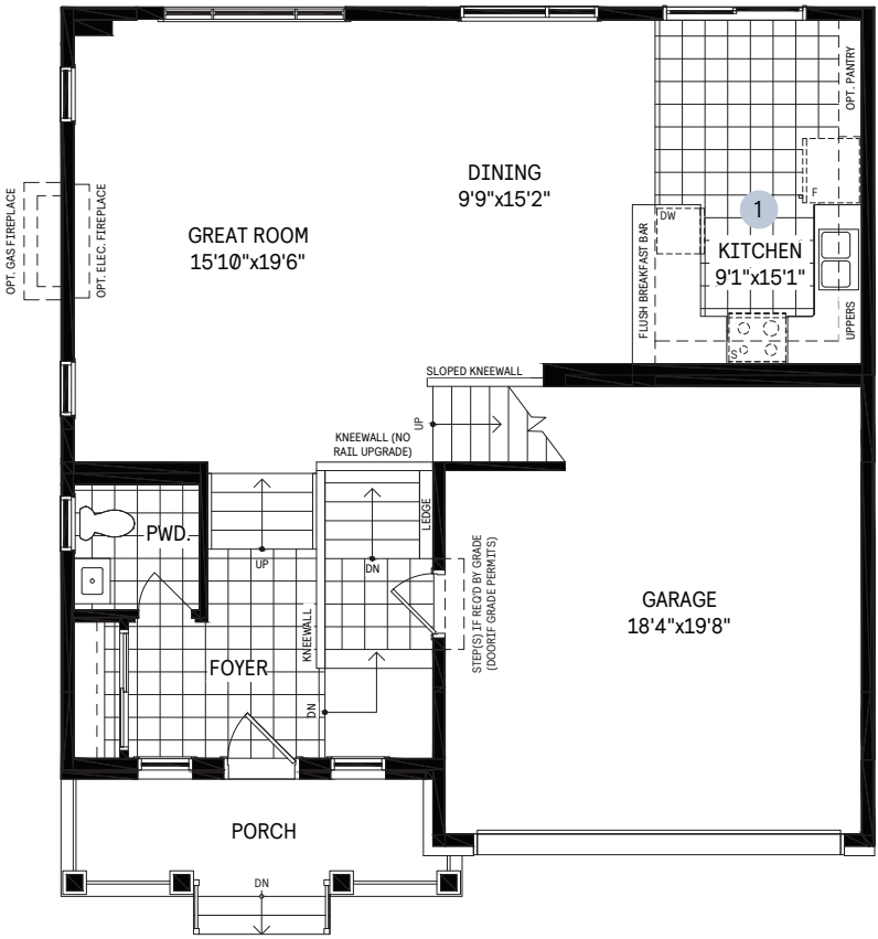
MAIN FLOOR
