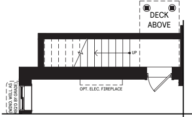
6 Optional Walk-Up Steps
