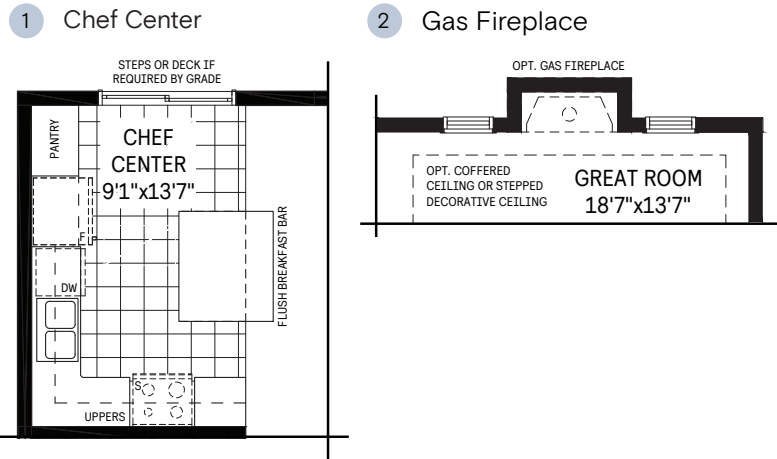
MAIN FLOOR – DESIGNER CHOICE OPTIONS
