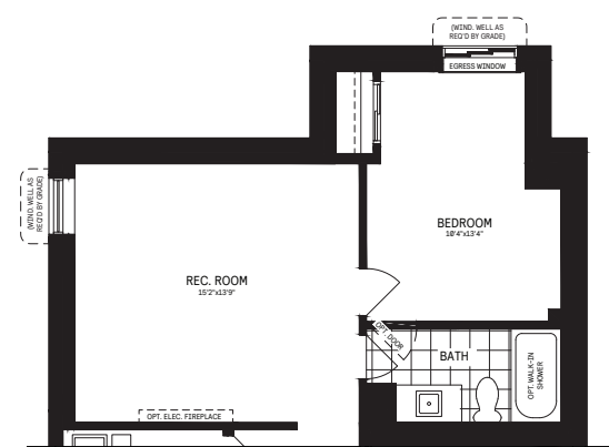
8C Finished Basement Package with Optional Walk-Up Steps
