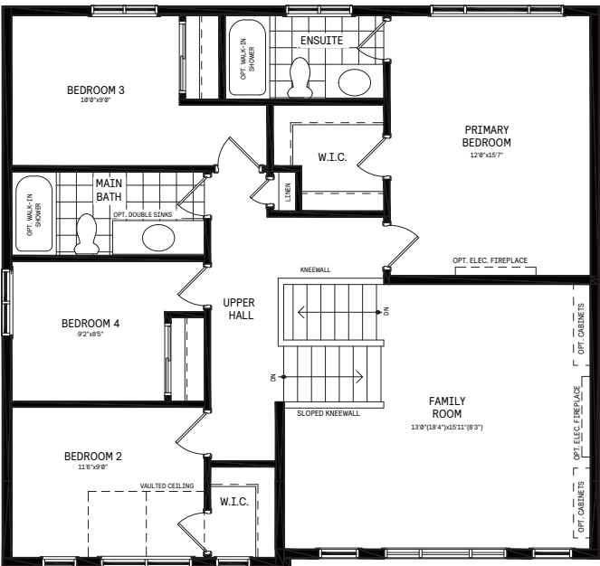
3 2nd Floor 4 Bedroom Plan
