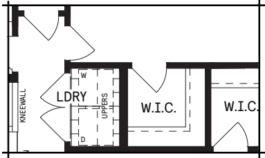
3 2nd Floor Laundry*
