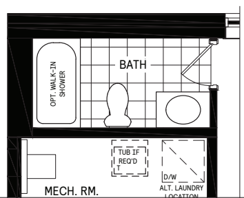
6 Finished Basement Bathroom
