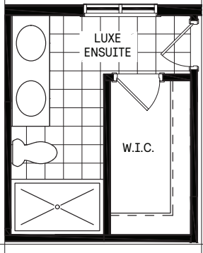
2 Second Floor Luxe Ensuite
