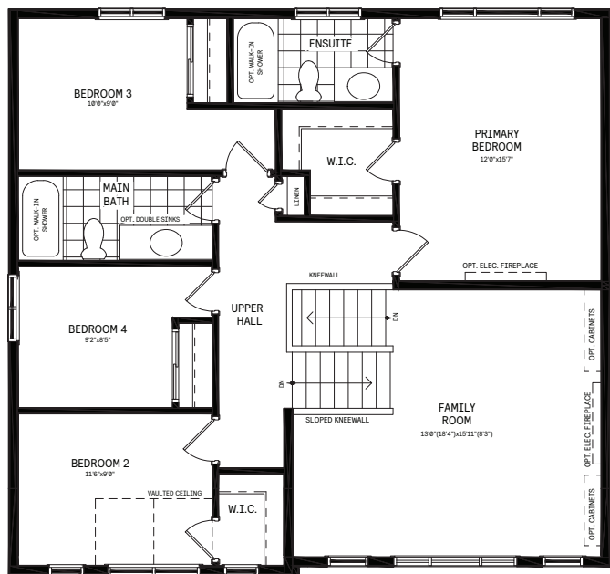
3 4 Bedroom Plan
