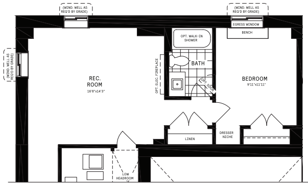
10 Finished Basement Package
