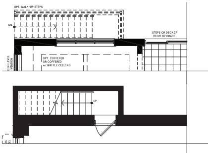
2 Optional Walk-up Steps
