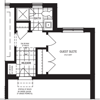
4 Main Floor Guest Suite
