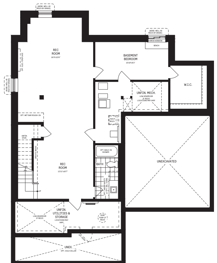
9 Finished Basement Package
