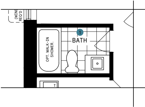
1 Finished Basement Bathroom
