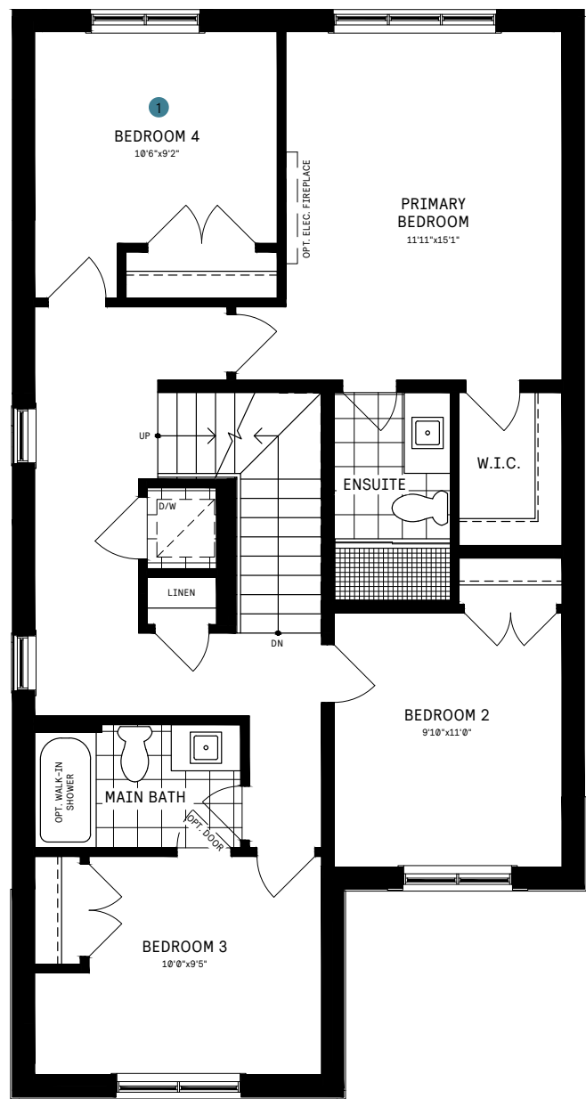
1 4 Bedroom Plan
