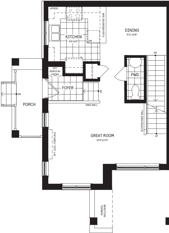
MAIN FLOOR
