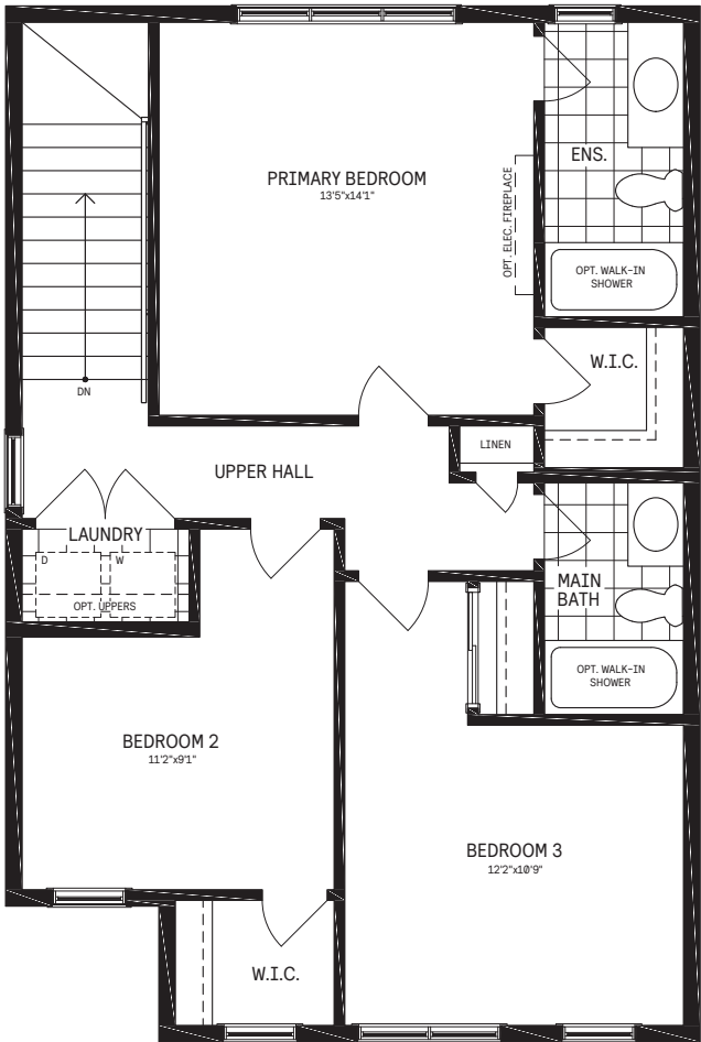
3 3 Bedroom Plan
