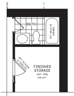
8 Finished Basement Bathroom
