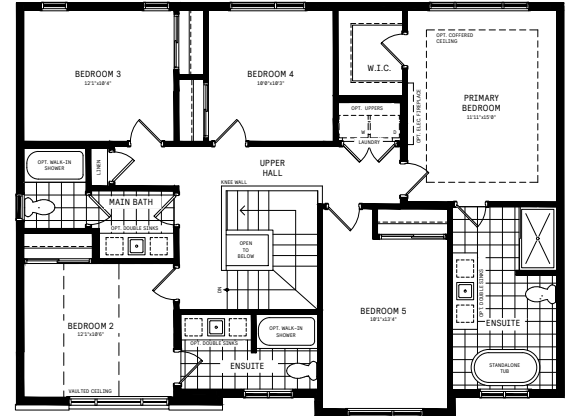
3 5 Bedroom Plan w/ Bedroom 2 Ensuite
