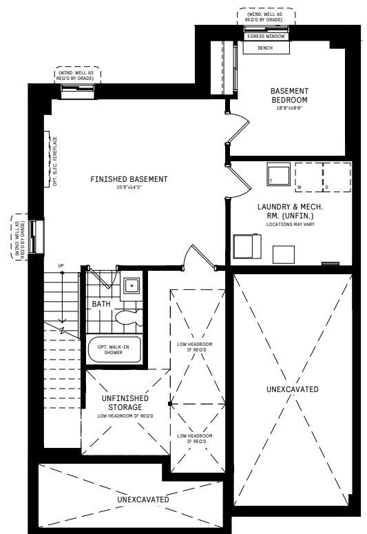
8 Finished Basement Package
