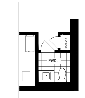
6 Finished Basement Powder Room
