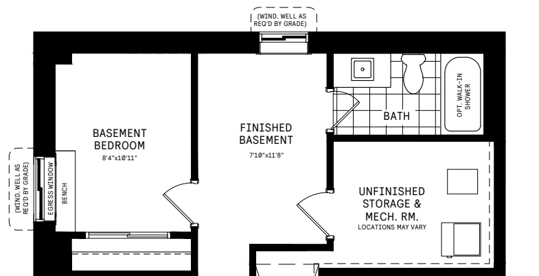
10 Finished Basement Package
