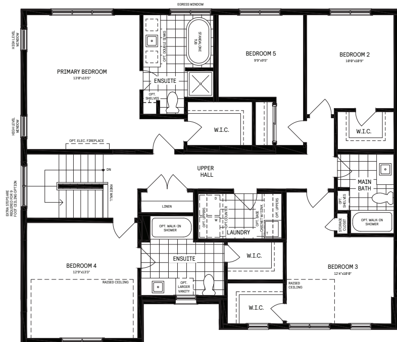
3 5 Bedroom Plan*
