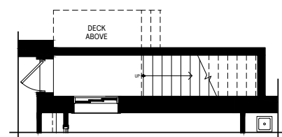
9C Finished Basement Package with Optional Walk-Up Steps
