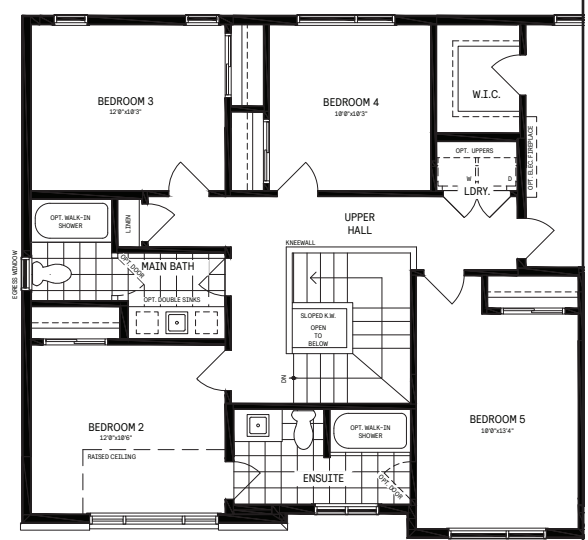
4 5 Bedroom Plan with Bedroom 2 Ensuite
