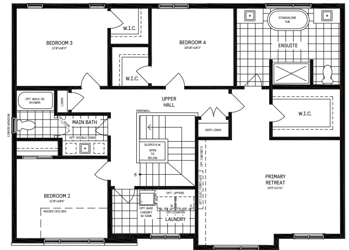
8A Optional Walk-Up Steps
