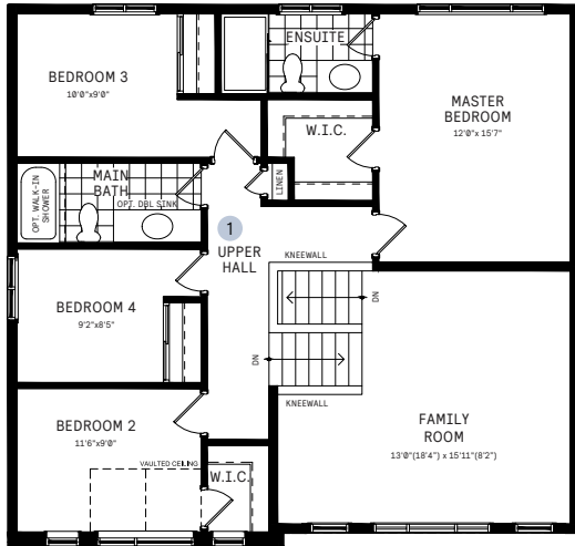
1 4 Bedroom Plan (Laundry relocated to Basement)
